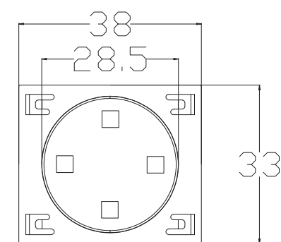
Product size
